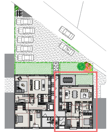
INPLANTINGSPLAN
